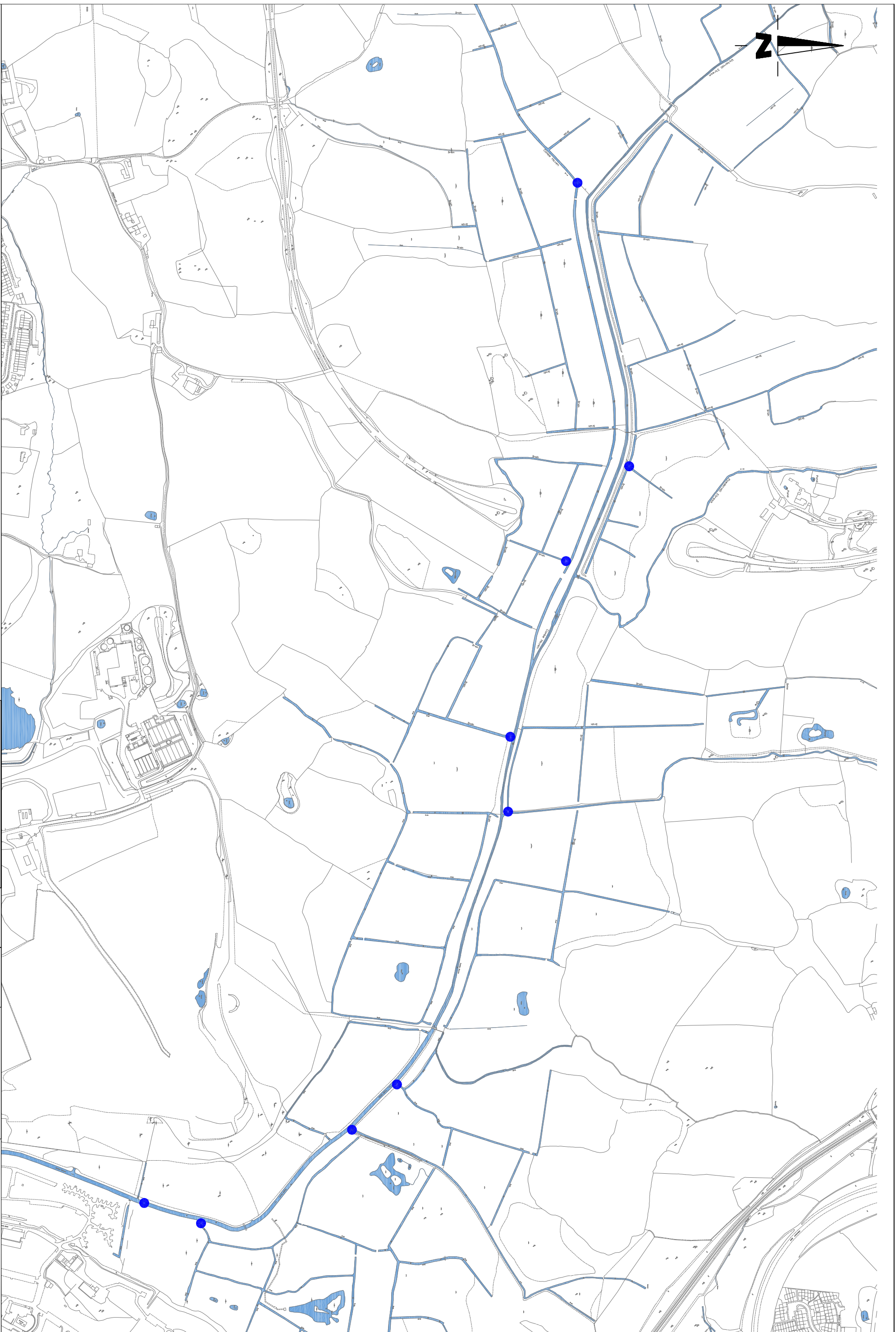
Figure : 3A.45 COMBE HAVEN CATCHMENT - STRUCTURES PROPOSED POSITION OF STOPLOGS
